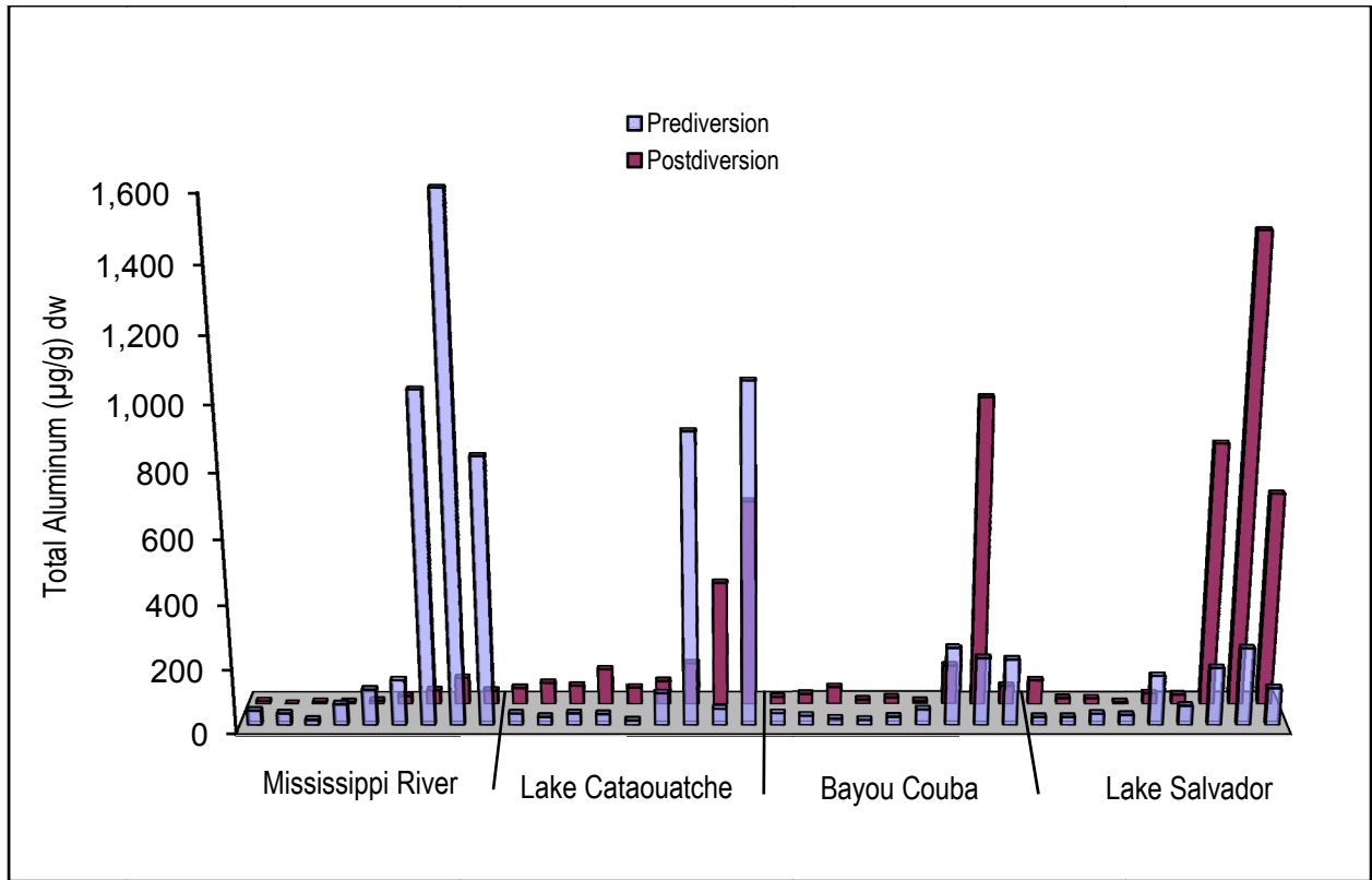
Figure 9B. Three-dimensional comparison of Davis Pond prediversion and postdiversion values for aluminum by dry weight (in micrograms per gram [ \mu\text{g/g} ]).
